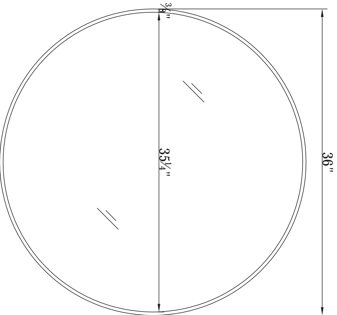
Front view
